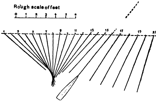
Fig. 6. Motion of an Oar during a Stroke. (Boat is moving towards the right hand.)
